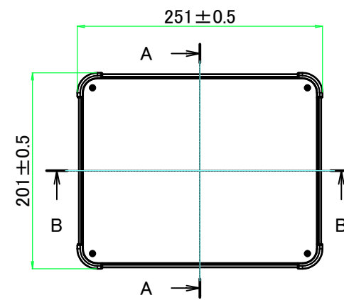
E view
